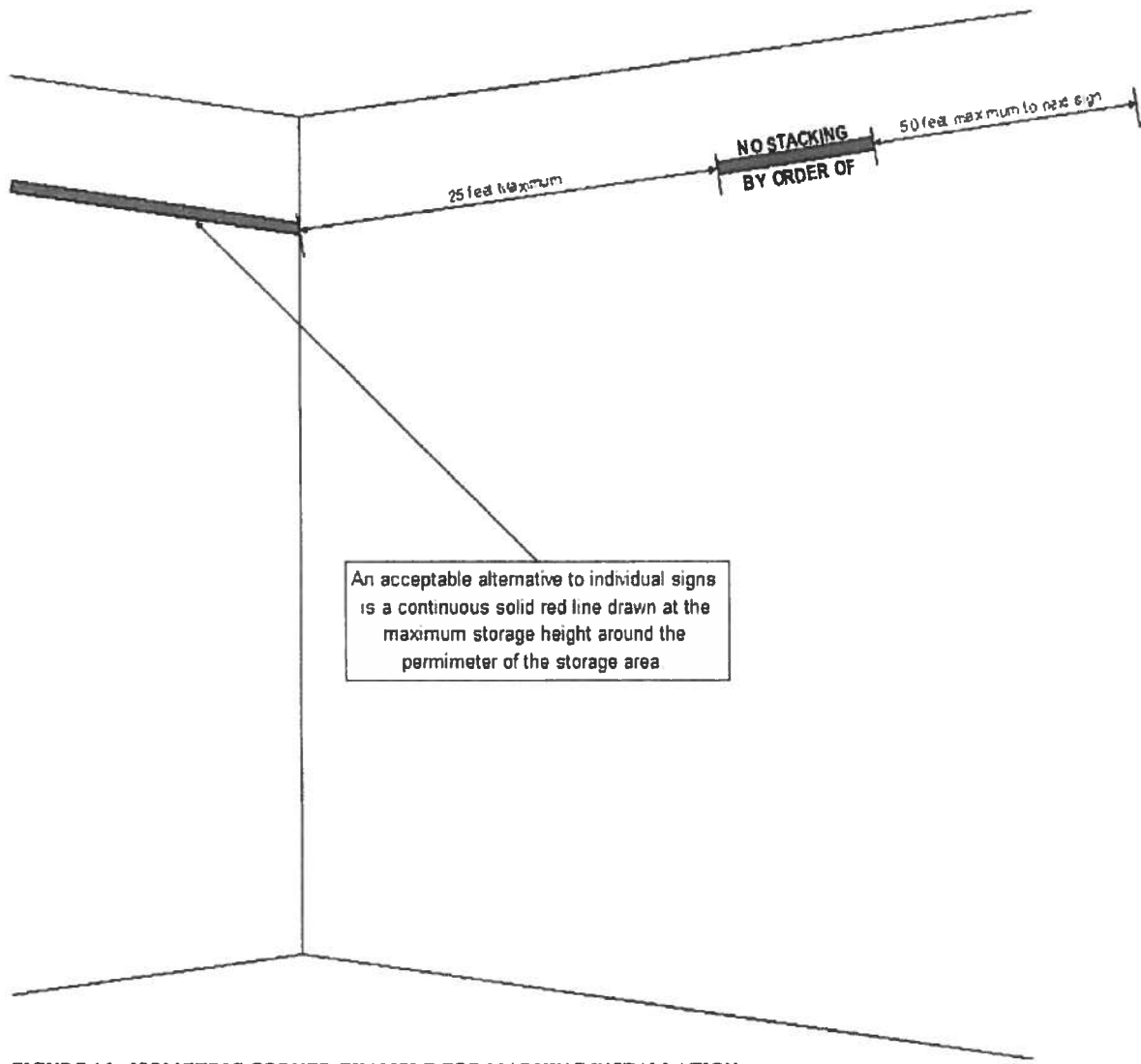
FIGURE 16 - ISOMETRIC CORNER EXAMPLE FOR MARKING INSTALLATION
