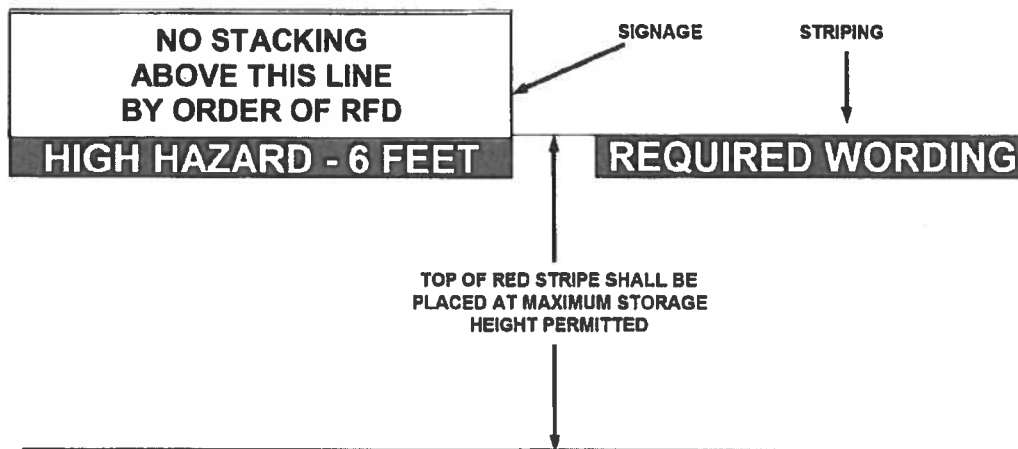
FIGURE 15 - SIGNAGE AND STRIPING VERTICAL INSTALLATION EXAMPLE
