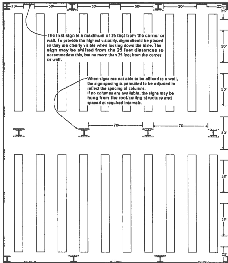
FIGURE 17 - SIGNAGE PLACEMENT AND SPACING EXAMPLE
