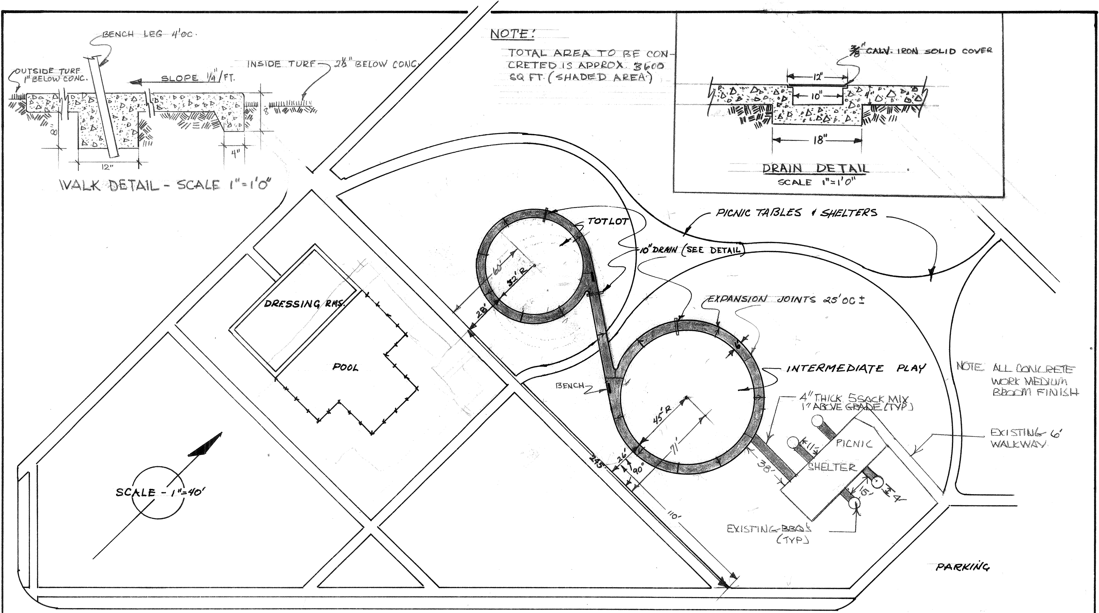
PROPOSED SITE PLAN HUNT PARK PLAYLAND CITY OF RIVERSIDE - PARK & RECREATION DEPT. 4-21-60
