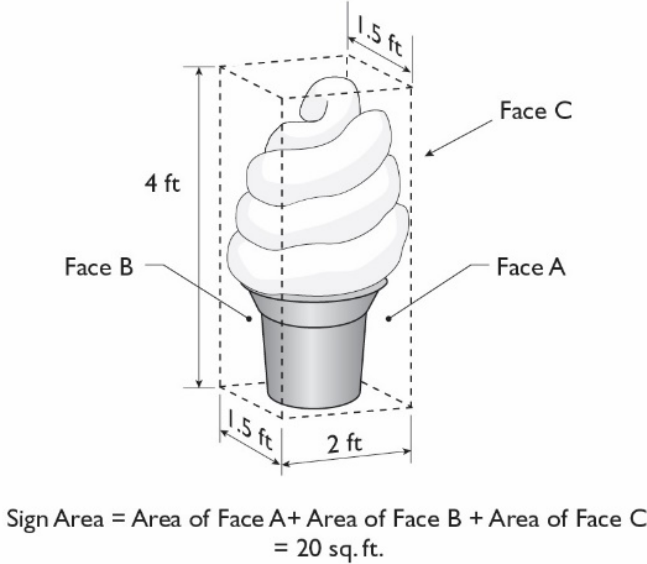
FIGURE 19.620.070.R-3: MEASURING AREA OF THREE-DIMENSIONAL SIGNS
