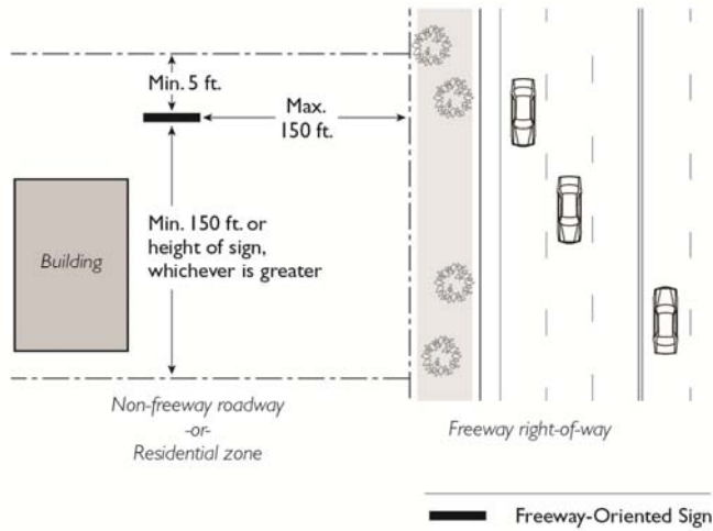
FIGURE 19.620.080.B-7: STANDARDS FOR FREEWAY ORIENTED SIGNS
